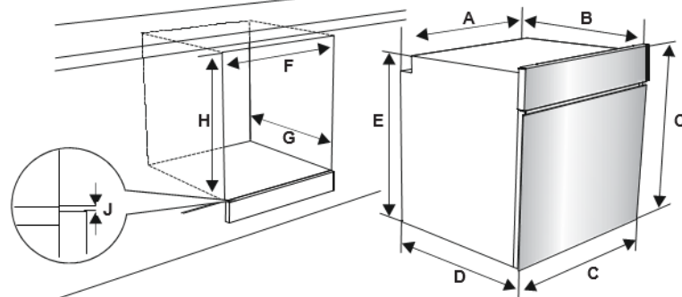
Installation under a worktop
